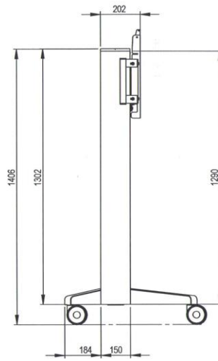
Technical drawing (mm) PR031010-P0 / SMS Presence Mobile
